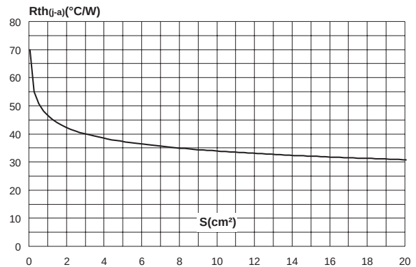
Fig. 12: Thermal resistance junction to ambient versus copper surface under tab (epoxy printed board FR4, Cu = 35μm)(D 2 PAK).
