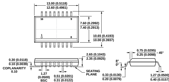
Figure 12. 16-Lead Standard Small Outline Package [SOIC_W] Wide Body (RW-16)
