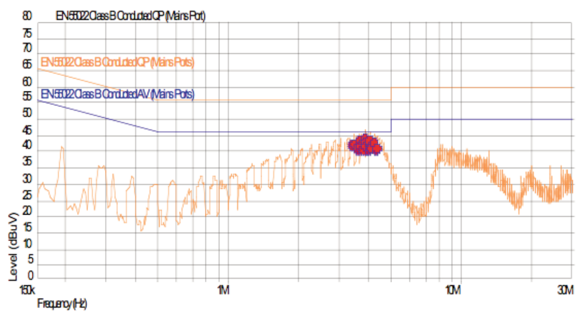
Figure 17 - QP Detector - LCL500PS48
