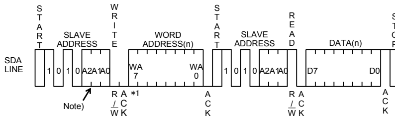
Fig.43 Random read cycle (BR24T01/02/04/08/16-W)
