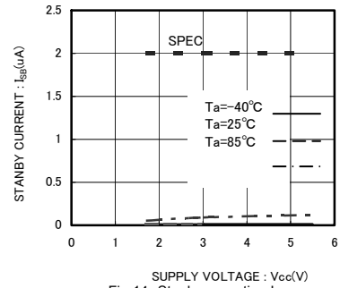
Fig.14 Standy operation I_{SSB} (fscI=400kHz BR24T01/02/04/08/16/32/64/128/256-W)
