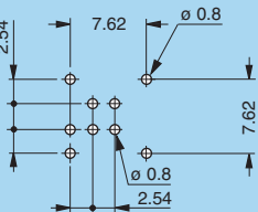
P19 - EPG-EXG (0B/1B.305) Solder mount
