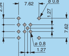
P19 - EPG-EXG (0B/1B.307) Solder mount
