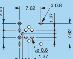
P19 - EPG-EXG (0B.309) Solder mount
