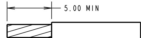
POWER CABLE STRIPPING DIMENSIONS
