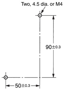
Mounting Holes
