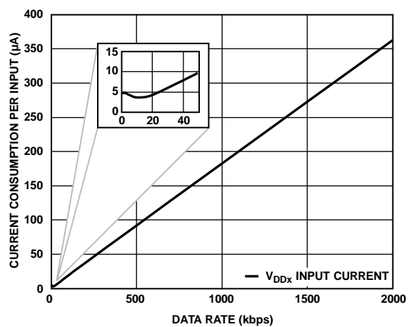
Figure 11. Current Consumption per Input vs. Data Rate for 3.3 V, EN_x = Low Operation
