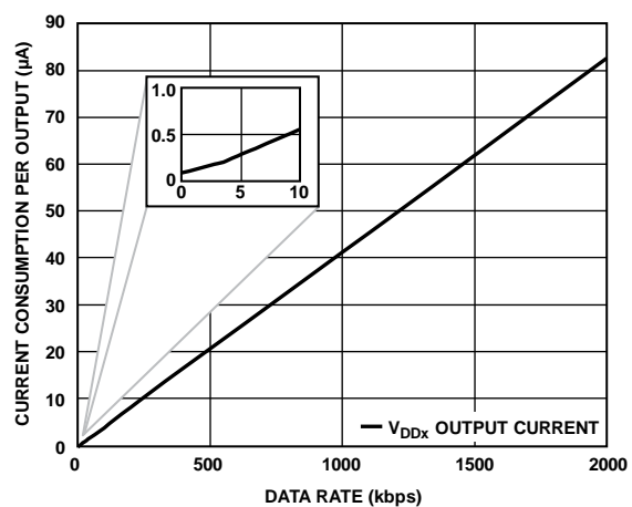
Figure 14. Current Consumption per Output vs. Data Rate for 2.5 V, EN_x = High Operation
