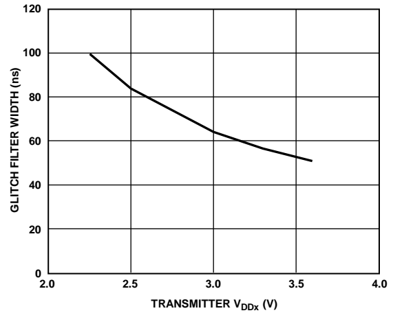
Figure 24. Typical Glitch Filter Operation Threshold
