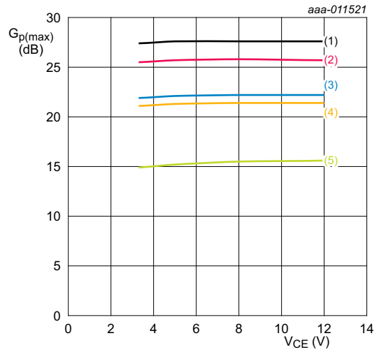
I_C = 15 \text{ mA} ; T_{amb} = 25 \text{ }^\circ\text{C} . If K > 1 then G_{p(max)} = maximum power gain. If K < 1 then G_{p(max)} = MSG. (1) f = 300 \text{ MHz} (2) f = 433 \text{ MHz} (3) f = 800 \text{ MHz} (4) f = 900 \text{ MHz} (5) f = 1800 \text{ MHz}
