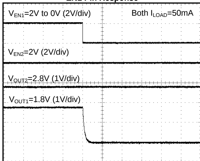
EN1 Pin Response
