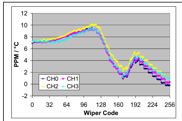
FIGURE 2-60: 50 kΩ – R_{WB} PPM/ ^\circ\text{C} vs. Wiper Setting. ( R_{BW(\text{code}=n, 125^\circ\text{C})}-R_{BW(\text{code}=n, -40^\circ\text{C})})/R_{BW(\text{code} = 256, 25^\circ\text{C})}/165^\circ\text{C} * 1,000,000 ) ( V_{DD} = 3.0\text{V} , I_W = 48\ \mu\text{A} ).
