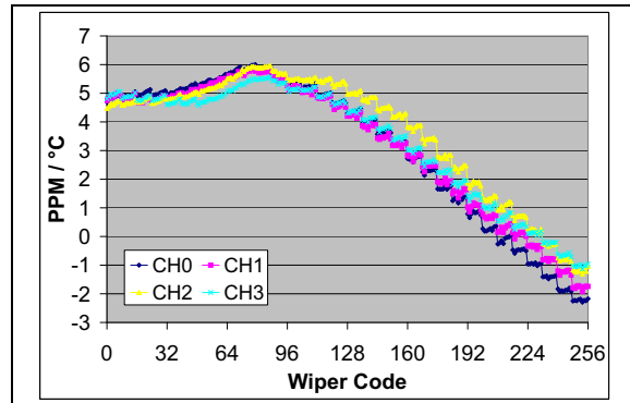
FIGURE 2-59: 50 kΩ – R_{WB} PPM/ ^\circ\text{C} vs. Wiper Setting. ( R_{BW(\text{code}=n, 125^\circ\text{C})}-R_{BW(\text{code}=n, -40^\circ\text{C})})/R_{BW(\text{code} = 256, 25^\circ\text{C})}/165^\circ\text{C} * 1,000,000 ) ( V_{DD} = 5.5\text{V} , I_W = 90\ \mu\text{A} ).
