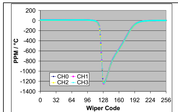
FIGURE 2-60: 50 kΩ – R_{WB} PPM/ ^\circ\text{C} vs. Wiper Setting. ( R_{BW(\text{code}=n, 125^\circ\text{C})}-R_{BW(\text{code}=n, -40^\circ\text{C})})/R_{BW(\text{code} = 256, 25^\circ\text{C})}/165^\circ\text{C} * 1,000,000 ) ( V_{DD} = 3.0\text{V} , I_W = 48\ \mu\text{A} ).
