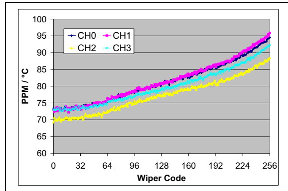
FIGURE 2-19: 5\text{ k}\Omega – R_{WB} PPM/ ^\circ\text{C} vs. Wiper Setting. ( R_{BW(\text{code}=n, 125^\circ\text{C})}-R_{BW(\text{code}=n, -40^\circ\text{C})})/R_{BW(\text{code} = 256, 25^\circ\text{C})}/165^\circ\text{C} * 1,000,000 ) ( V_{DD} = 3.0\text{V} , I_W = 190\ \mu\text{A} ).
