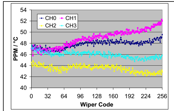
FIGURE 2-18: 5\text{ k}\Omega – R_{WB} PPM/ ^\circ\text{C} vs. Wiper Setting. ( R_{BW(\text{code}=n, 125^\circ\text{C})}-R_{BW(\text{code}=n, -40^\circ\text{C})})/R_{BW(\text{code} = 256, 25^\circ\text{C})}/165^\circ\text{C} * 1,000,000 ) ( V_{DD} = 5.5\text{V} , I_W = 190\ \mu\text{A} ).
