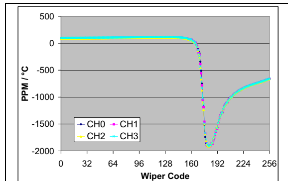
FIGURE 2-19: 5\text{ k}\Omega – R_{WB} PPM/ ^\circ\text{C} vs. Wiper Setting. ( R_{BW(\text{code}=n, 125^\circ\text{C})}-R_{BW(\text{code}=n, -40^\circ\text{C})})/R_{BW(\text{code} = 256, 25^\circ\text{C})}/165^\circ\text{C} * 1,000,000 ) ( V_{DD} = 3.0\text{V} , I_W = 190\ \mu\text{A} ).
