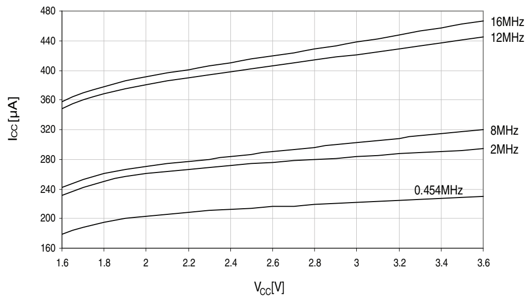
Figure 33-262. Standby Supply Current vs. V_{CC} T = 25^{\circ}C , running from different crystal oscillators
