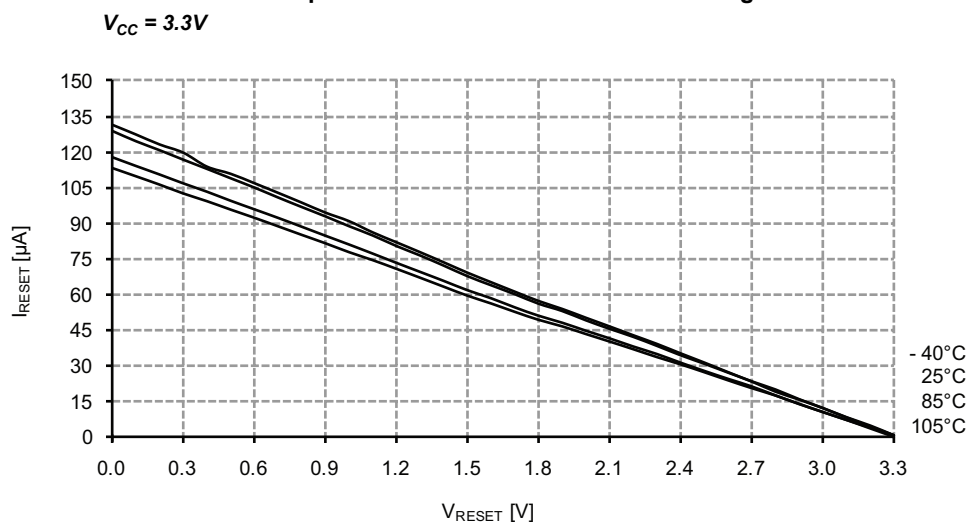
Figure 33-223. Reset Pin Pull-up Resistor Current vs. Reset Pin Voltage
