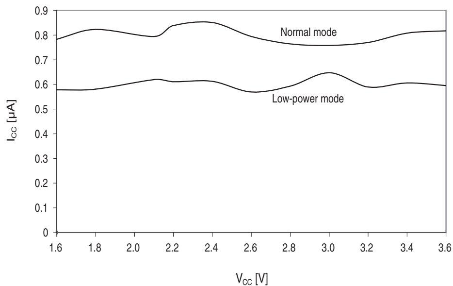
Figure 33-97. Power-save Mode Supply Current vs. V_{CC}
