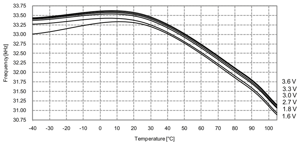
Figure 33-312. Ultra Low-Power Internal Oscillator Frequency vs. Temperature
