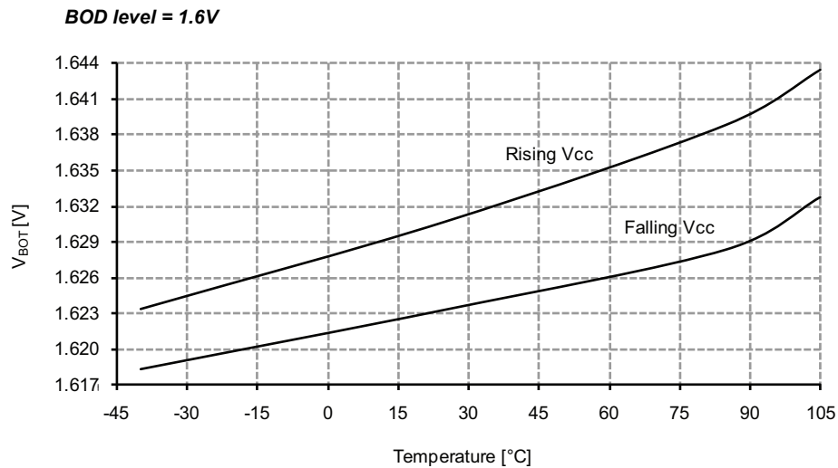
Figure 33-218. BOD Thresholds vs. Temperature
