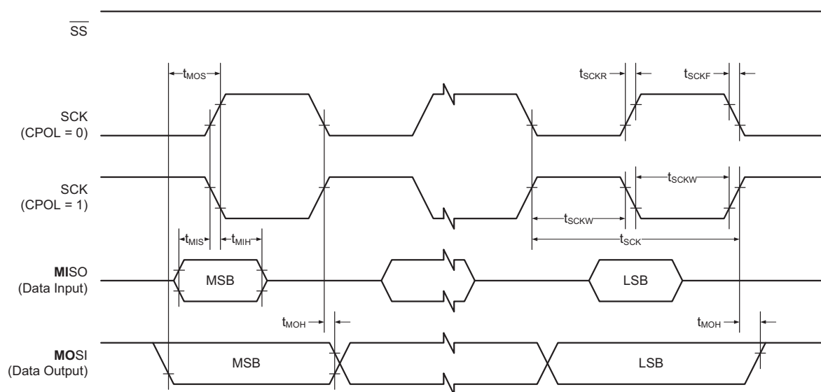
Figure 32-5. SPI Timing Requirements in Master Mode
