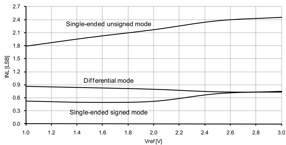
Figure 33-194. INL Error vs. External V_{REF} T = 25^\circ\text{C} , V_{CC} = 3.6\text{V} , external reference
