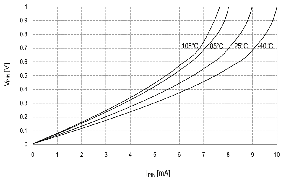
Figure 33-107. I/O Pin Output Voltage vs. Sink Current
