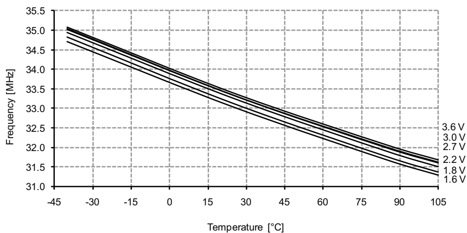
Figure 33-234. 32MHz Internal Oscillator Frequency vs. Temperature
