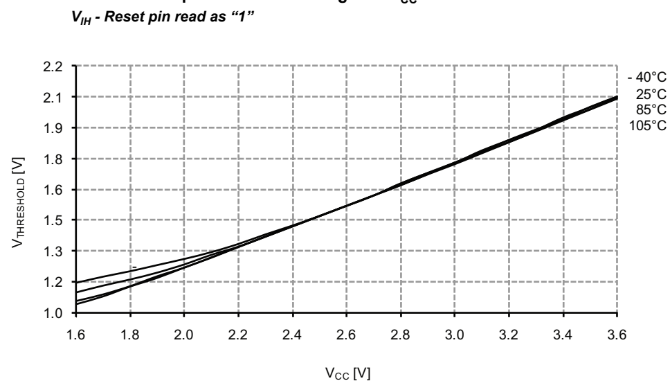
Figure 33-224. Reset Pin Input Threshold Voltage vs. V_{CC}
