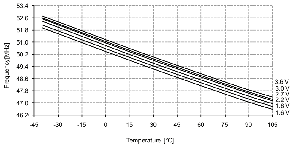
Figure 33-238. 48MHz Internal Oscillator Frequency vs. Temperature
