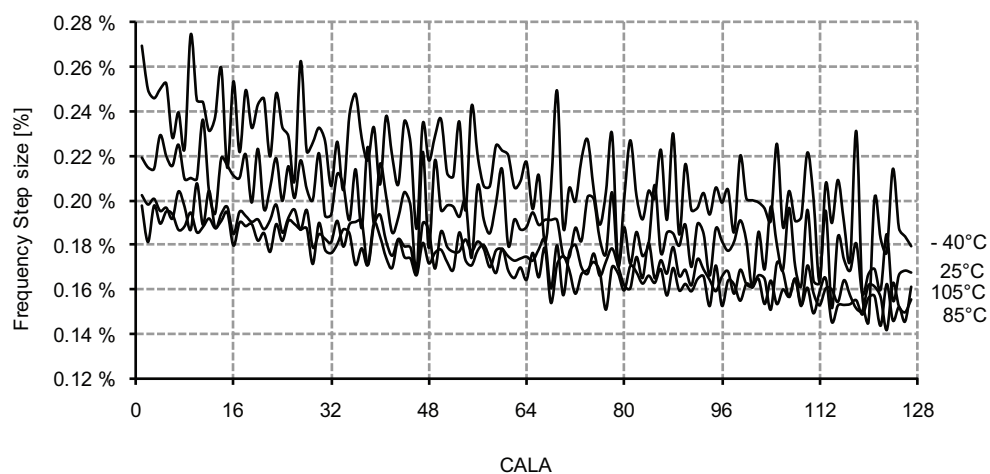
Figure 33-233. 2MHz Internal Oscillator CALA Calibration Step Size
