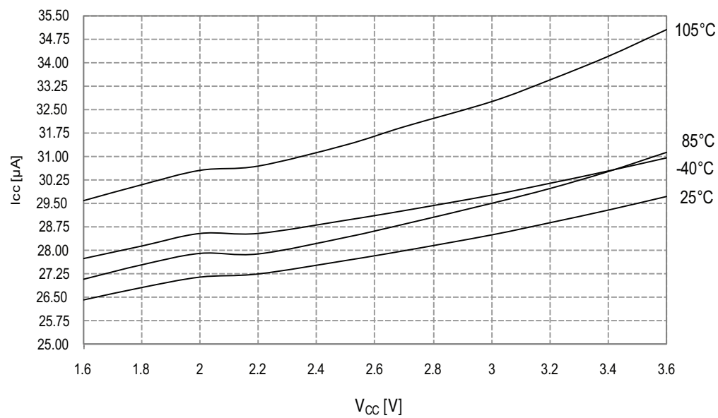
Figure 33-89. Idle Mode Supply Current vs. V_{\text{CC}}
