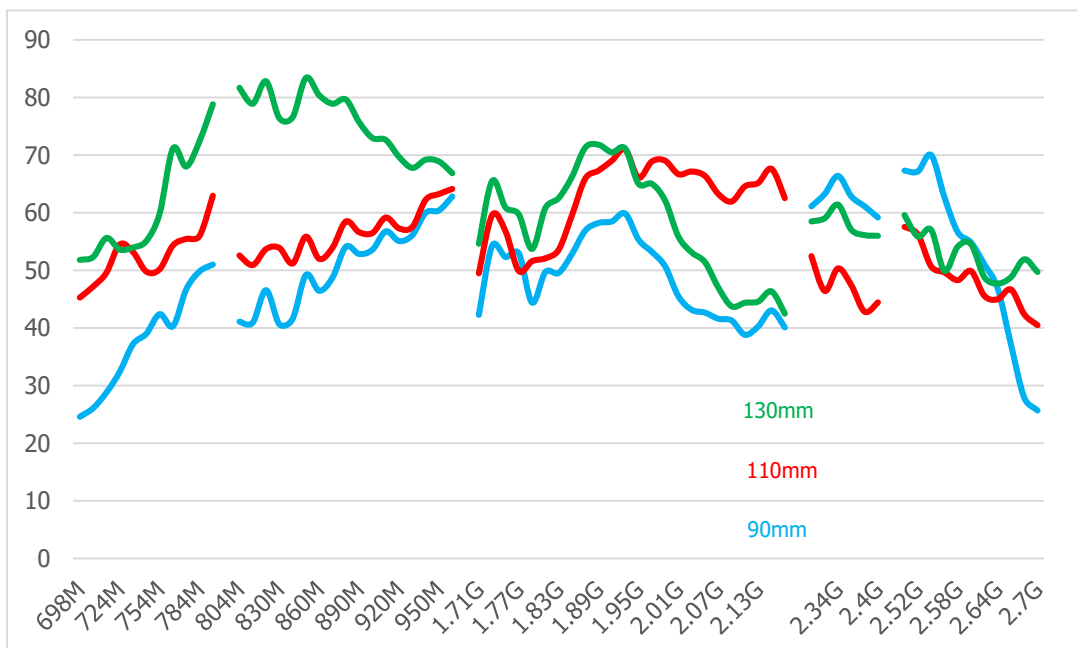
Passive Efficiency vs. PCB length All results measured in Antenova's anechoic chamber
