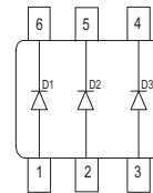
BAT68-08S
