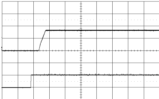
Start-up enabled by connecting V_I at: T_{P1} = +25^{\circ}\text{C} , V_I = 12\text{ V} , V_O = 3.3\text{ V} C_O = 470\text{ }\mu\text{F}/10\text{ m}\Omega , I_O = 12\text{ A} Top trace: output voltage (2 V/div.). Bottom trace: CTRL signal (2 V/div.). Time scale: (20 ms/div.).
