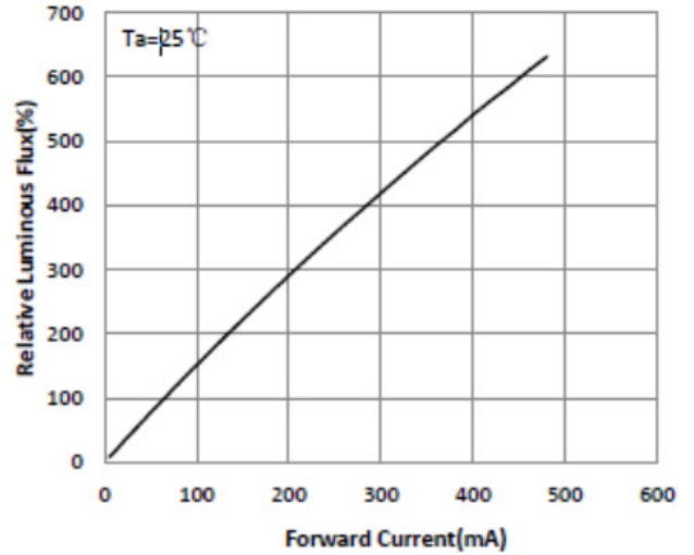
I_f ----- Relative Luminous flux
