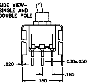
PRINTED CIRCUIT MOUNTING
