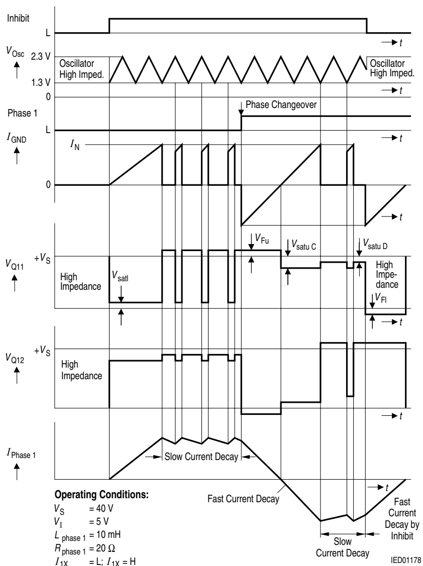
Figure 10 Phase Reversal and Inhibit
