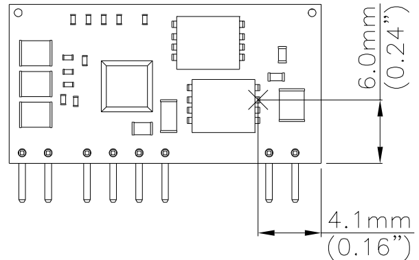
Figure 25: Temperature measurement location* The allowed maximum hot spot temperature is defined at 130
