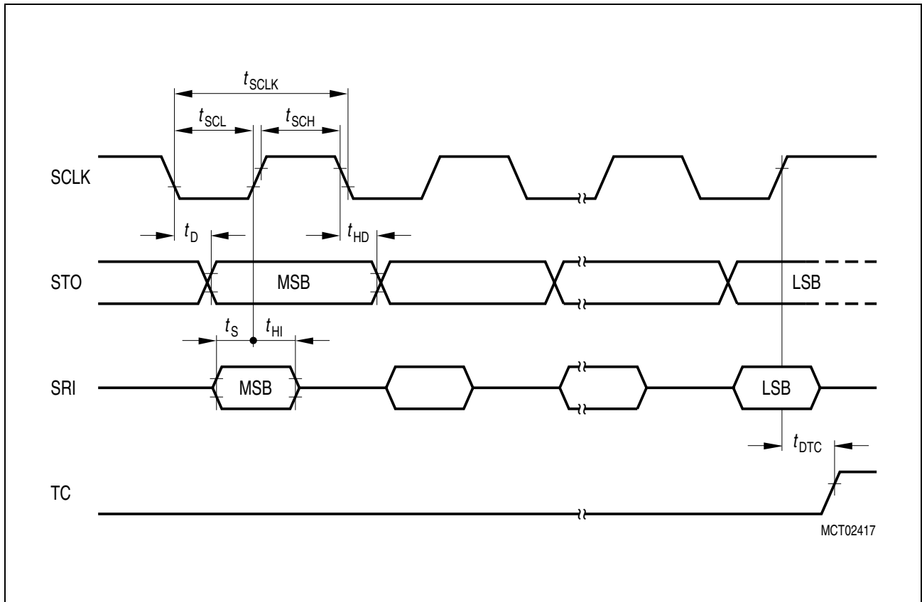
Figure 34 SSC Timing
