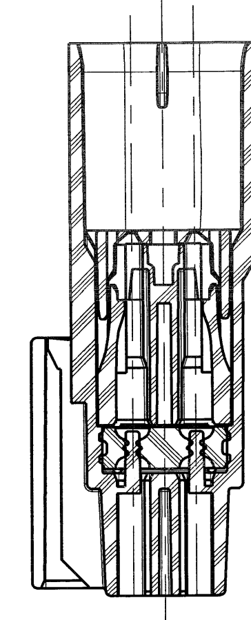
T.P.A IN PRE-ASSEMBLED POSITION
