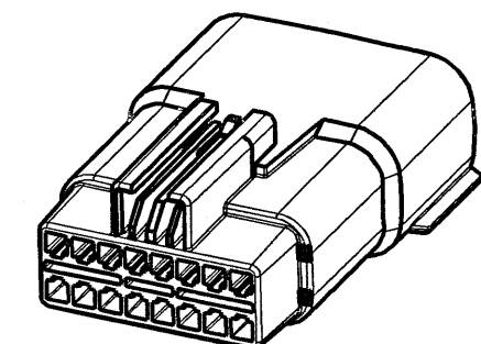
MALE HOUSING SHOWING CLIP SLOT OPTIONS CLIP SLOT TYPE-1 ACTUAL SIZE VIEWS
