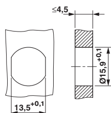
Housing cutout for M16 fastening thread, mounting panel with feed-through hole
