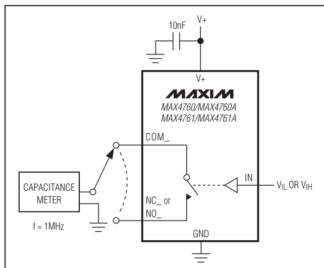
Figure 7. Channel On-/Off-Capacitance
