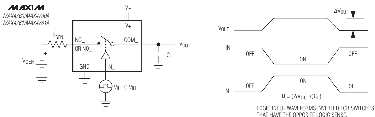
Figure 5. Charge Injection
