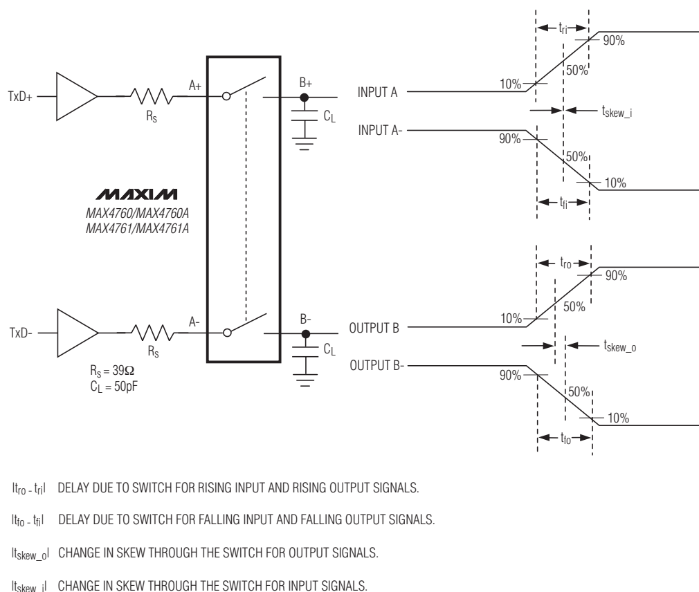
Figure 4. Input/Output Skew Timing Diagram
