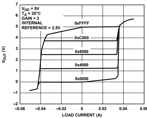
Figure 34. Source and Sink Capability at 5 V
