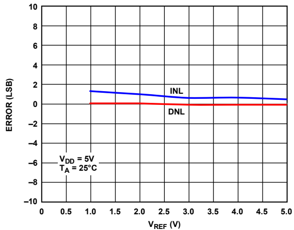
Figure 22. INL Error and DNL Error vs. V_{REF}
