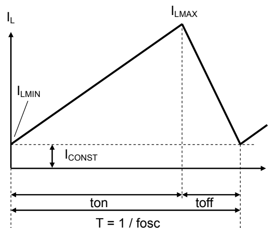
Figure 4. Continuous Mode
