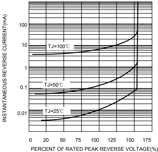
FIG.3-TYPICAL REVERSE CHARACTERISTICS
