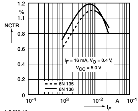
Fig. 13 - Current Transfer Ratio (Normalized) vs. Forward Current
