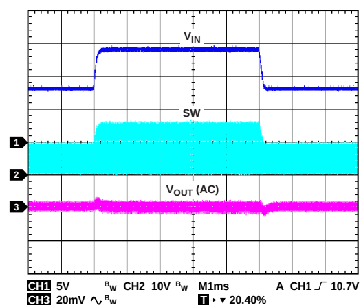
Figure 28. Line Transient Response, V_{IN} from 8 V to 14 V, I_{OUT} = 1 A
