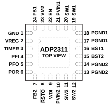
Figure 4. Pin Configuration
