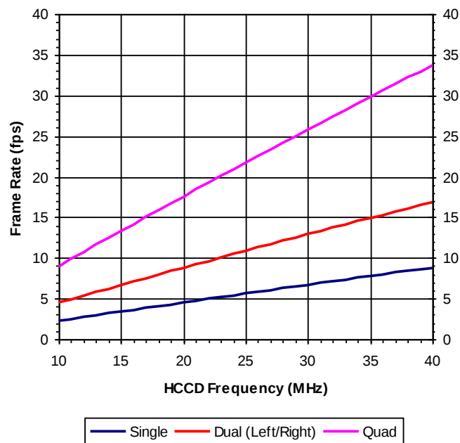
Figure 12: Frame Rates
