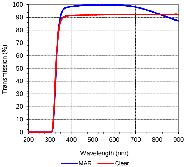
Figure 27: Cover Glass Transmission
