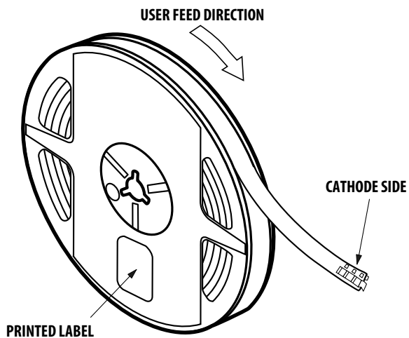
Figure 12. Reeling Orientation.
