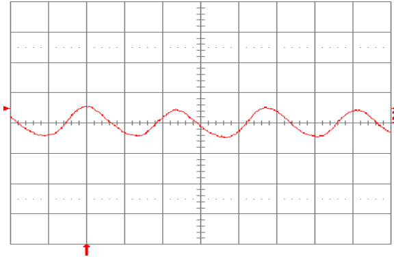
Fig. 3.3V.15: Input reflected ripple current, i_c (100 mA/div.), measured at input terminals at full rated load current and V_{in} = 24\text{V} . Refer to Fig. 3.3V.14 for test setup. Time scale: 1 \mu\text{s}/\text{div} .
