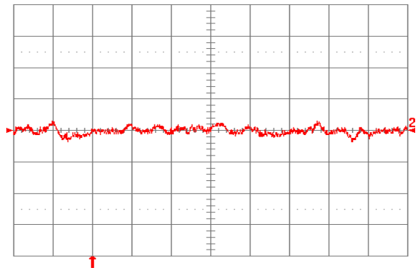
Fig. 1.8V.16: Input reflected ripple current, i_s (10 mA/div.), measured through 10 \mu\text{H} at the source at full rated load current and V_{in} = 24 \text{ V} . Refer to Fig. 1.8V.14 for test setup. Time scale: 1 \mu\text{s}/\text{div} .
