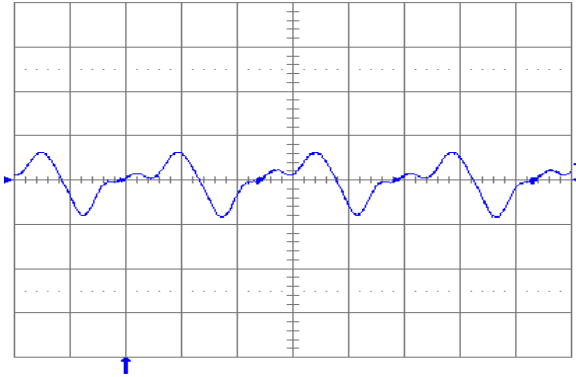
Fig. 1.8V.13: Output voltage ripple (20 mV/div.) at full rated load current into a resistive load with C_o = 10 \mu\text{F} tantalum + 1\mu\text{F} ceramic and V_{in} = 24 \text{ V} . Time scale: 1 \mu\text{s}/\text{div} .
