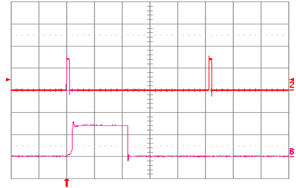
Fig. 5.0V.18: Load current (top trace, 10 A/div., 20 ms/div.) into a 10 mΩ short circuit during restart, at Vin = 24V. Bottom trace (10 A/div., 1 ms/div.) is an expansion of the on-time portion of the top trace.
