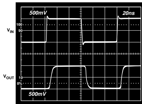
Figure 20. Small Signal Pulse Response, Gain = +1, ( R_F = 2k\Omega , R_L = 150\Omega , V_S = \pm 5V )
