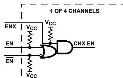
FIGURE 5. ISL32179E ENABLE LOGIC
