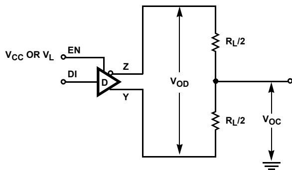
FIGURE 1. DC DRIVER TEST CIRCUITS
