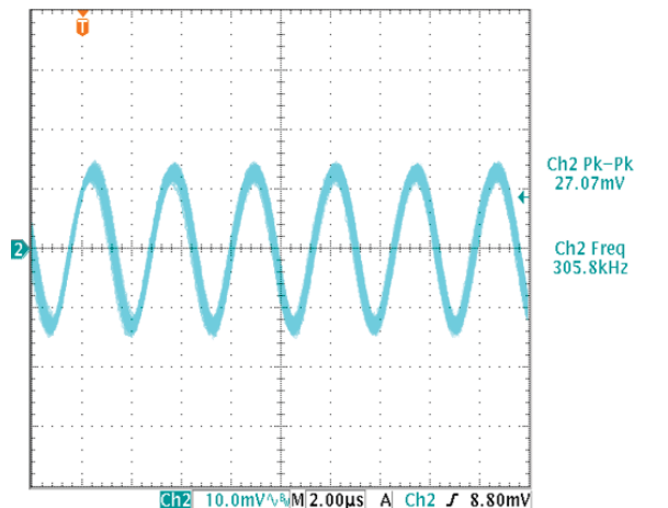
Output Ripple and Noise (Vin=5V, Iout=0A, Vout=3.3V, Cout= 1uF || 10uF, Ta=+25°C)
