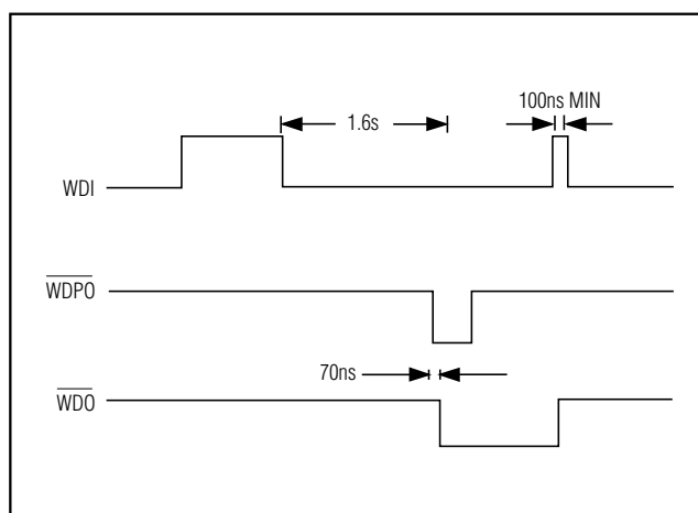
Figure 5. WDI, WDO, and WDPO Timing Diagram ( V_{\text{CC}} Mode)
