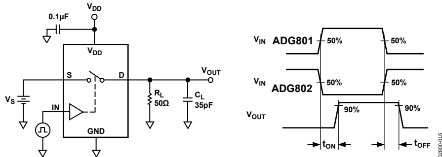
Figure 16. Switching Times
