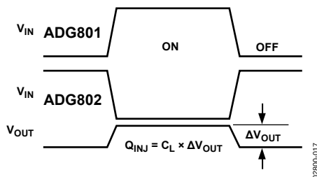
Figure 17. Charge Injection
