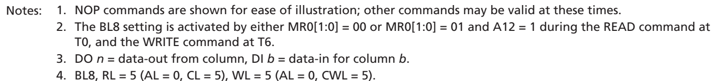
4Gb: x4, x8, x16 DDR3L SDRAM READ Operation
