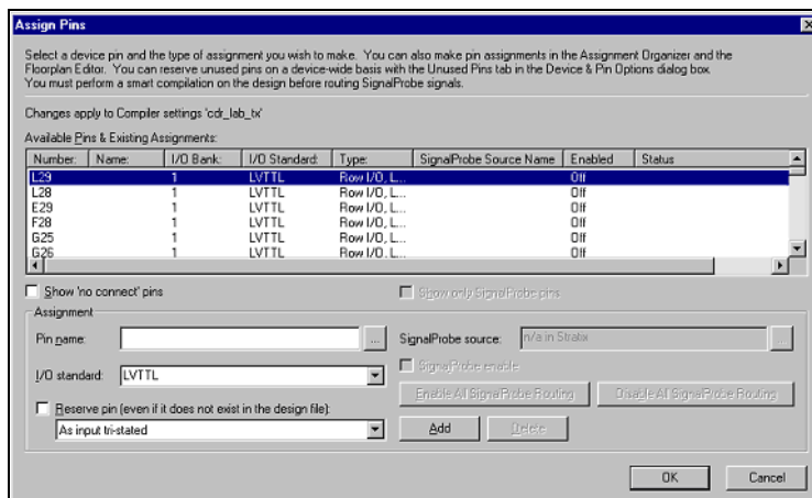
Figure 4-23. Assign Pins
