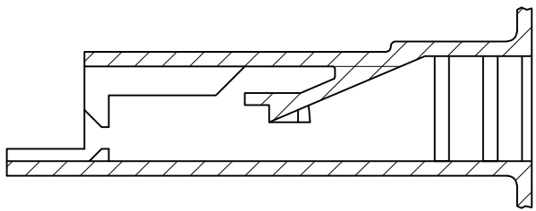
SECTION Y-Y ROTATED 85° CCW
