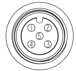
Conn.1 & Conn.2 Pin Assignments Front View
