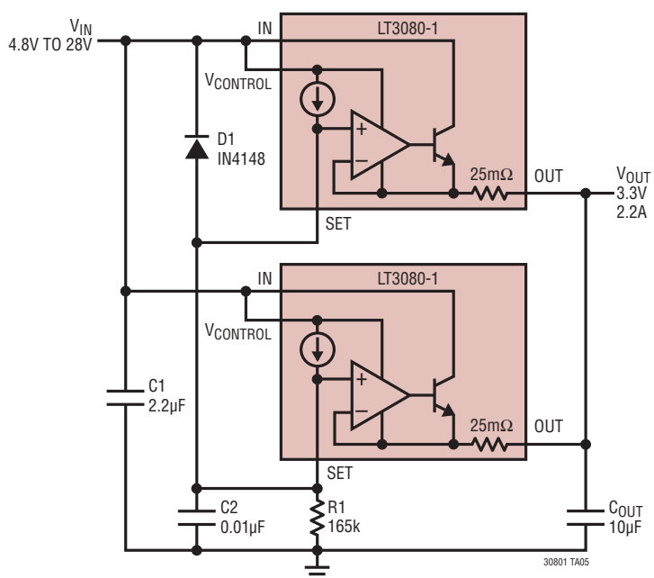
Adding Soft-Start
