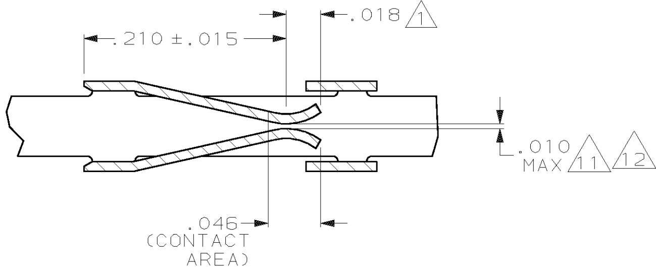
SECTION X-X
