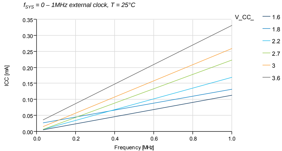
Figure 37-1. Active Mode Supply Current vs. Frequency
